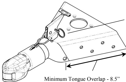
Retaining Pin
