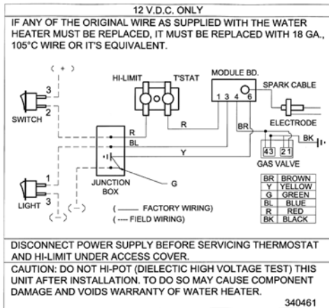
Figure 8 MAKING ELECTRICAL CONNECTIONS 120 VOLTS A.C.
